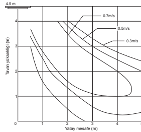
MMU-UP0361HP-TR, UP0481HP-TR, UP0561HP-TR (Yüksek tavan 3)
