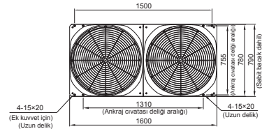
MMY-MAP1606FT8P-TR MMY-MAP1806FT8P-TR MMY-MAP2006FT8P-TR
